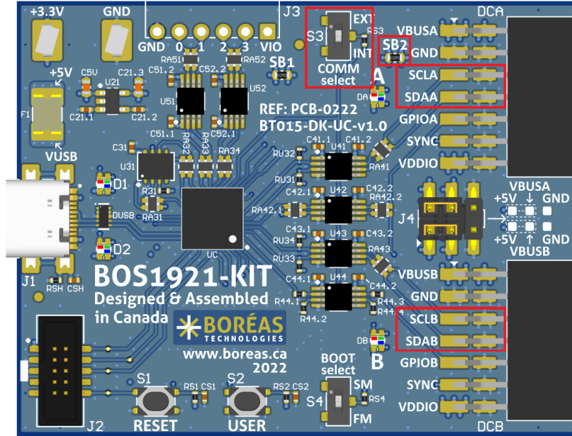
Figure 9: Comm selection switch and SPI header location
