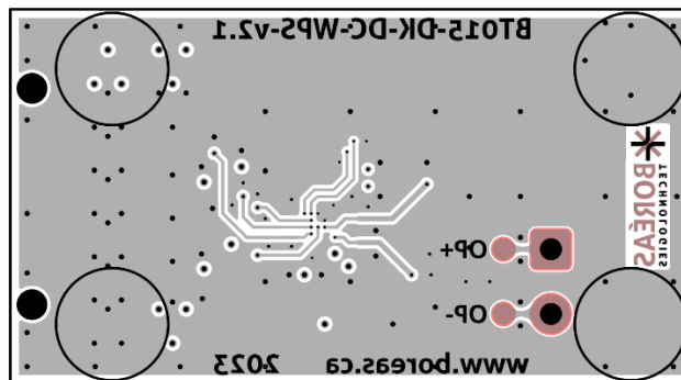
Figure 23: Layout view - Bottom Layer (not to scale)
