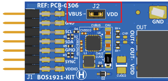
Figure 11: Driver board UPI mode configuration jumper location
