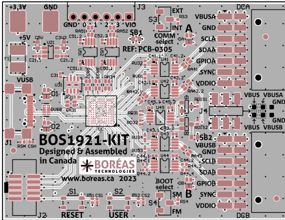
Figure 14: Layout view - Top Layer (not to scale)
