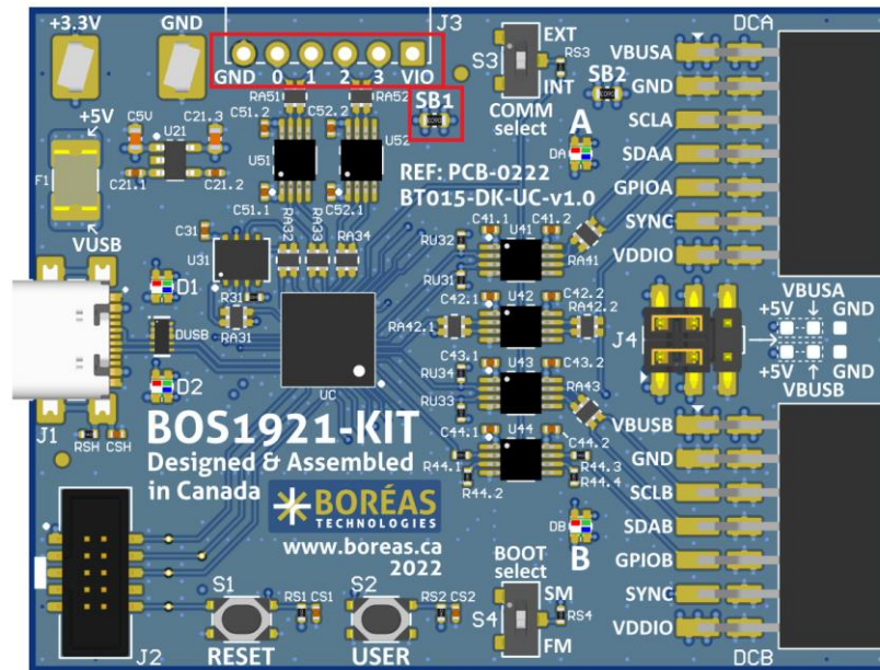
Figure 8: GPIOs and GPIOs supply voltage configuration solder bridge location
