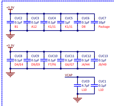
Microcontroller Caps
