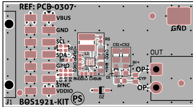
Figure 20: Layout view - Top Layer (not to scale)
