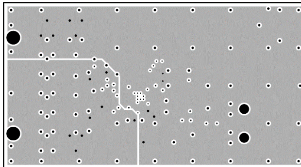
Figure 22: Layout view - Third Layer (not to scale)
