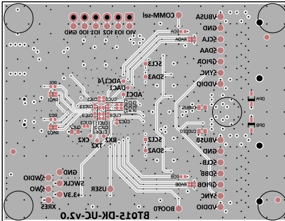
Figure 15: Layout view - Bottom Layer (not to scale)
