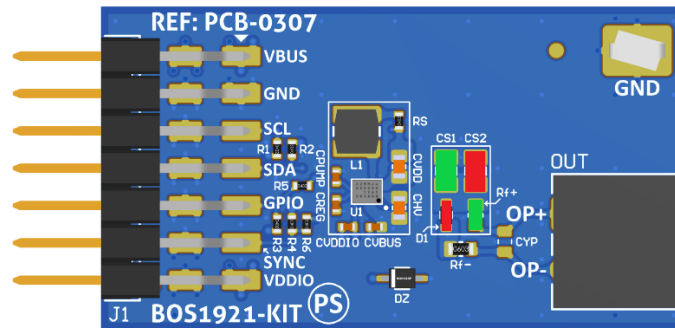
Figure 13: Pump driver board component reconfiguration for direct waveform output
