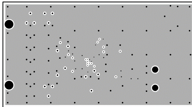
Figure 21: Layout view - Second Layer (not to scale)
