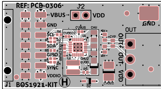
Figure 16: Layout view - Top Layer (not to scale)
