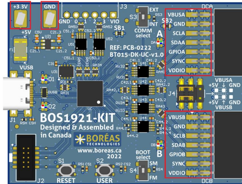
Figure 7: Probe hook location
