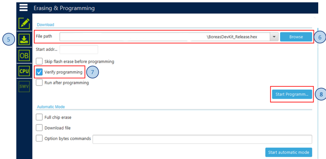
Figure 26: STM32CubeProgrammer programming setting
