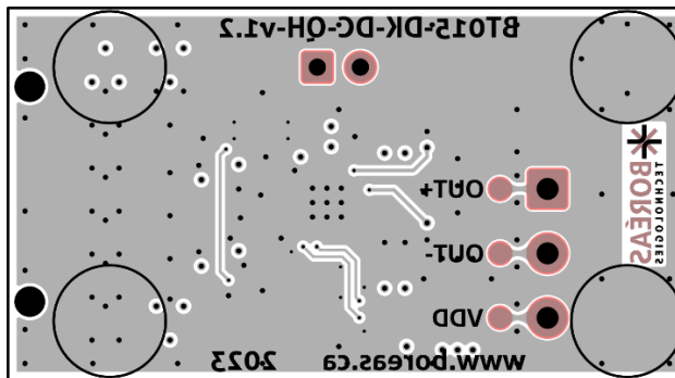
Figure 19: Layout view - Bottom Layer (not to scale)
