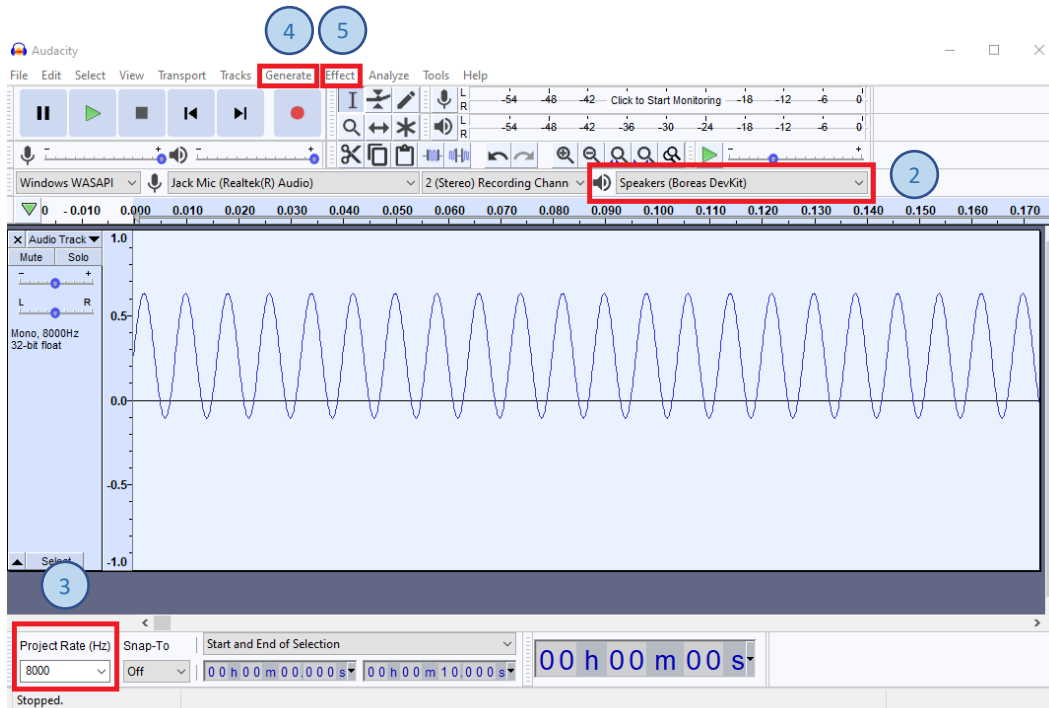
Figure 32: Audacity – simple waveform creation
