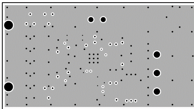
Figure 17: Layout view - Second Layer (not to scale)
