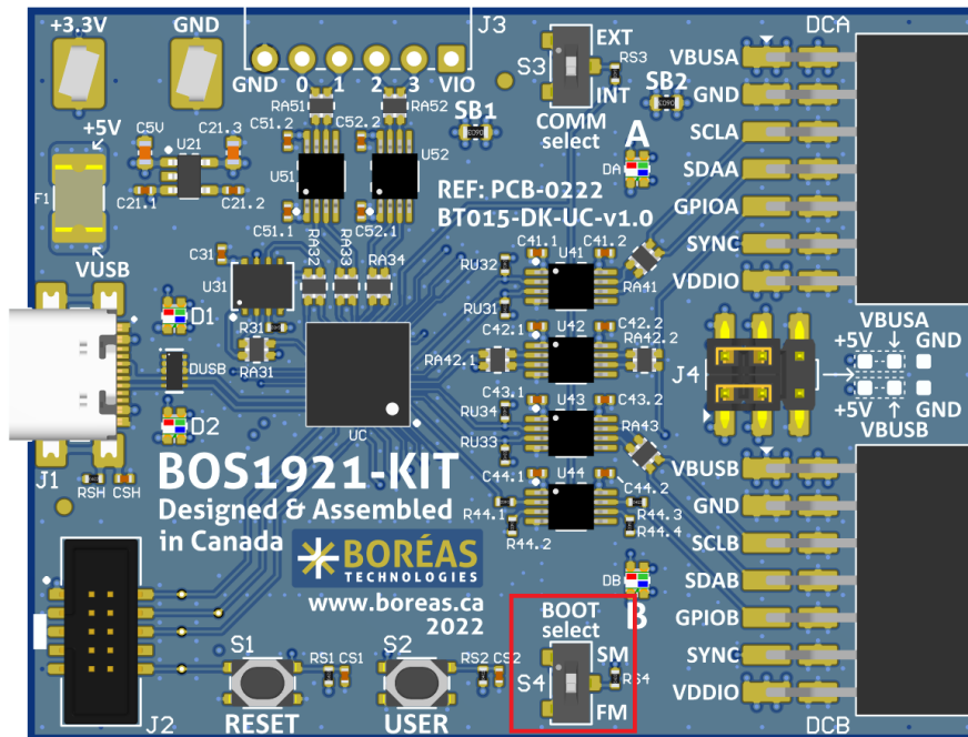
Figure 24 : Boot selection switch position
