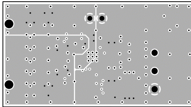
Figure 18: Layout view - Third Layer (not to scale)
