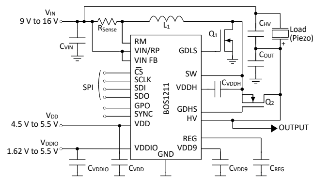
Figure 1: Simplified schematic
